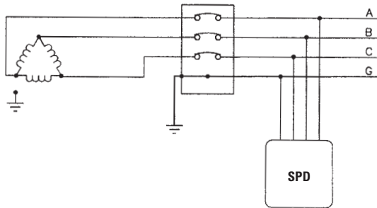
Fig. 1: 3-Phase, 3-Wire DELTA
