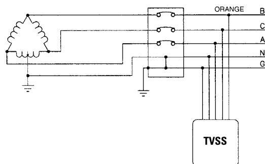
Fig. 5: 3-Phase, 4-Wire High-Leg DELTA
