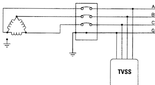
Fig. 5: 3-Phase, 4-Wire High-Leg DELTA
